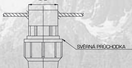
DETAIL PROSTUPU Ø D
